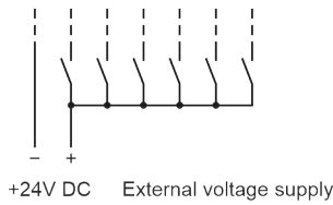
Voltage supply of RM-351 C / 310
