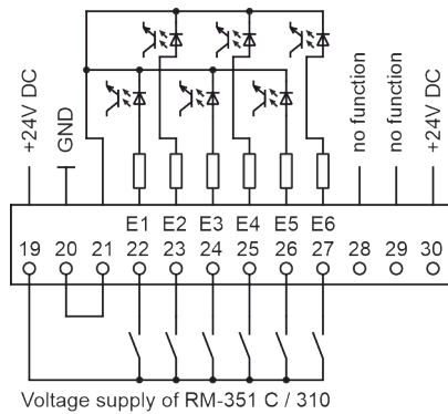
Voltage supply of RM-351 C / 310
