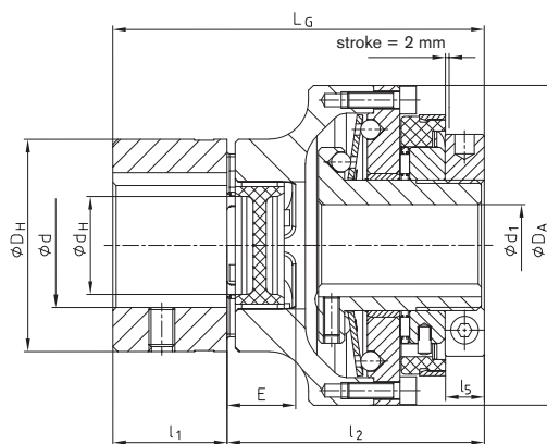
SYNTEX® - zero-backlash, torsionally rigid overload coupling with ROTEX® - GS
